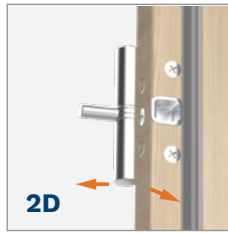
Hinges adjustable in two planes with caps matching fitting's colour
