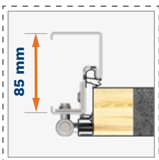
PERFOTHERM 50* steel door frame
